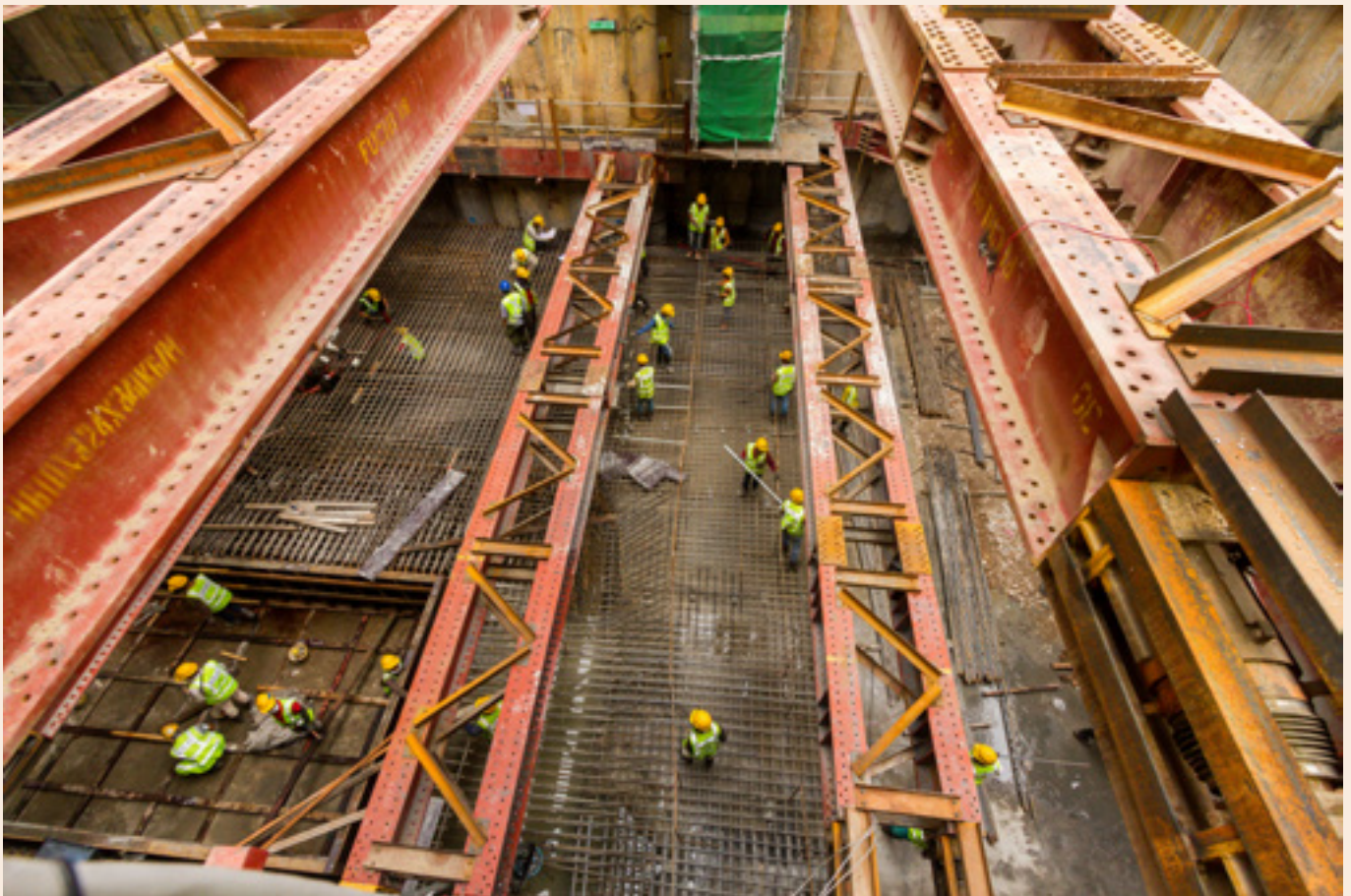
Construction of the Merdeka station.
