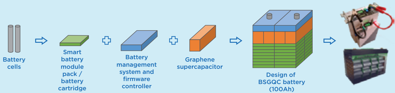
Structure of backup-storage graphene-based quantum cells (BSGQC).
